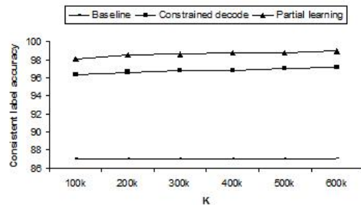
Figure 4: Wiki label evaluation results: Label
