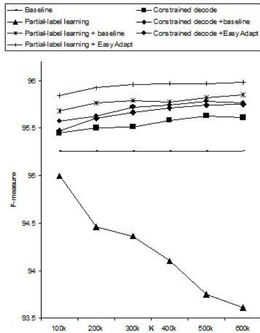
Figure 5: CTB evaluation results
