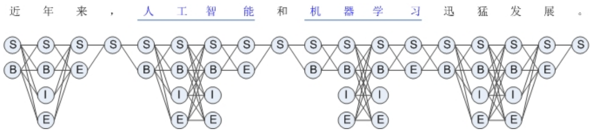
Figure 1: Sausage constraint (partial labels) from natural annotations and punctuation
