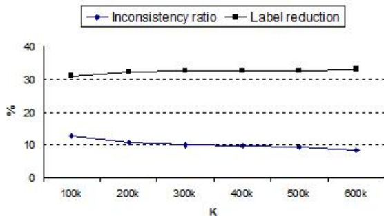
Figure 2: Encoded knowledge: inconsistency ratio and label reduction
