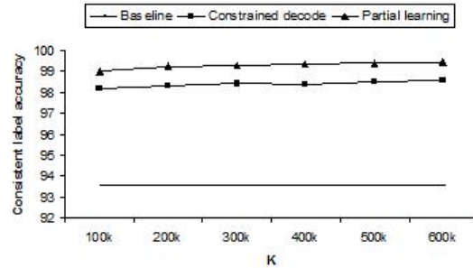
Figure 3: Wiki label evaluation results: Full
